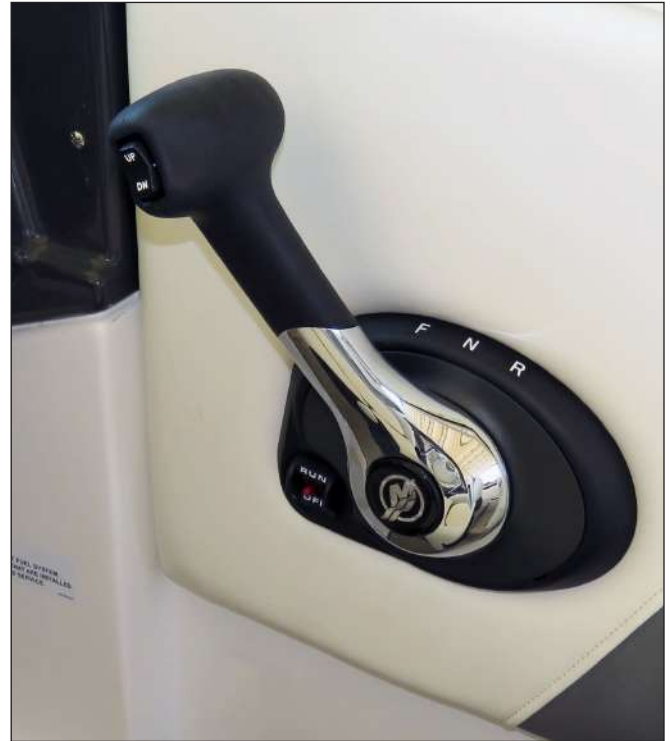
Typical Mercury Engine Side Mount Cable Control & Stop Switch
